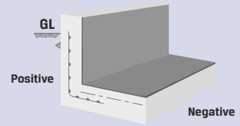
Below grade structures
